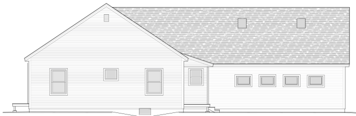
Left Elevation
